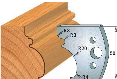
Pair of knives 690.501 Pair of limiters 691.501
