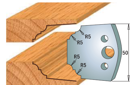
Pair of knives 690.580 Pair of limiters 691.580
