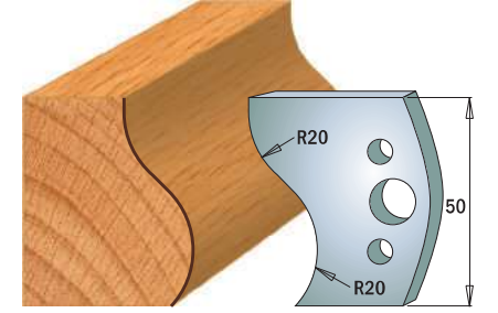
Pair of knives 690.571 Pair of limiters 691.571
